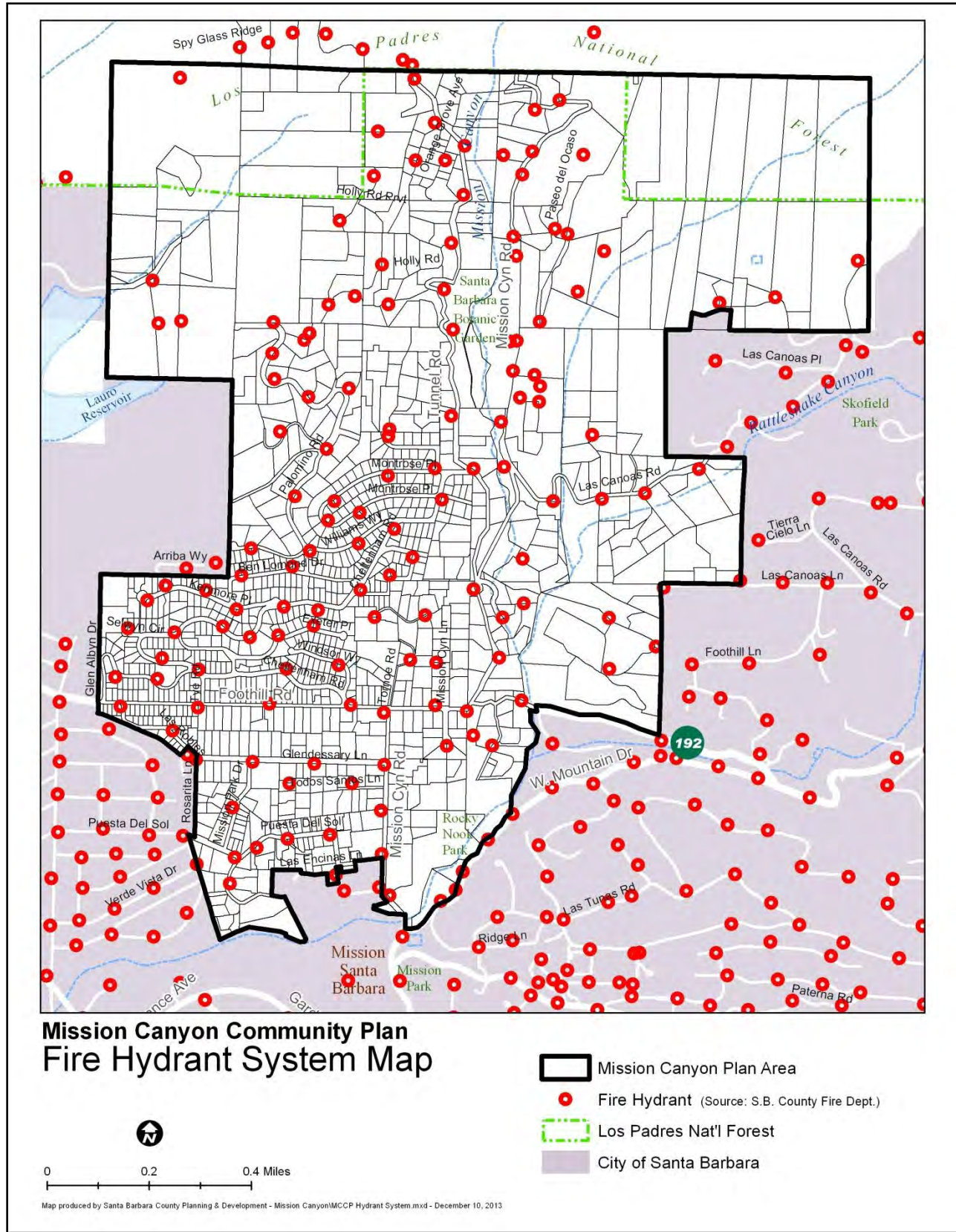
Figure 11: Fire Hydrant System (as of 2013)
